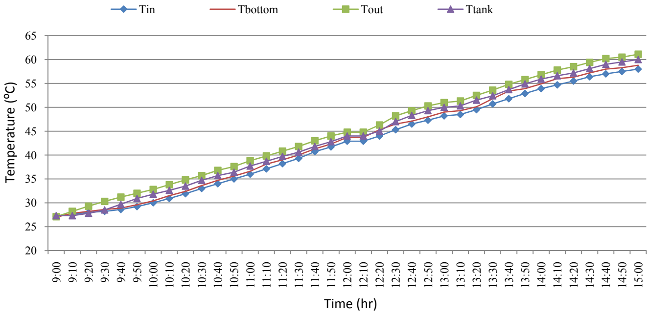
Fig. 10: Temperature of SWH1 at 22° on November 22, 2014
