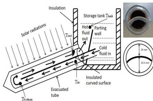
Fig. 8: Schematic diagram of SWH2
