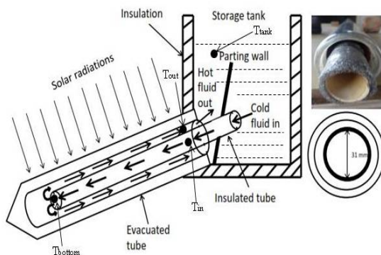
Fig. 9: Schematic diagram of SWH3
