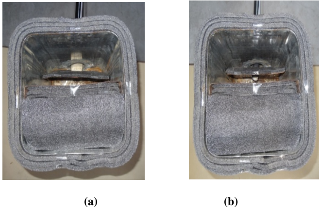
Fig. 3: (a) Photograph of curved insulated surface tank (b) Photograph of concentric circular insulated surface tank
