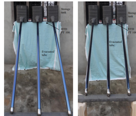
Fig. 1: Photograph of systems at 45^\circ and 22^\circ
