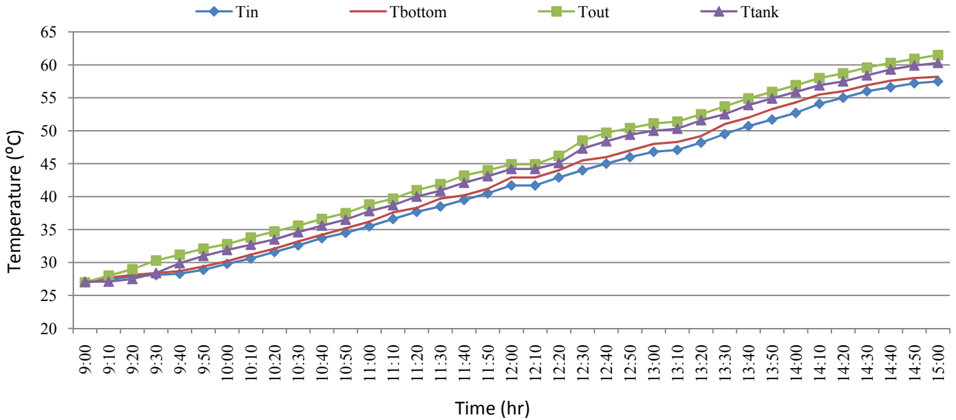
Fig. 11: Temperature of SWH2 at 22° on November 22, 2014
