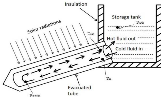
Fig. 7: Schematic diagram of SWH1
