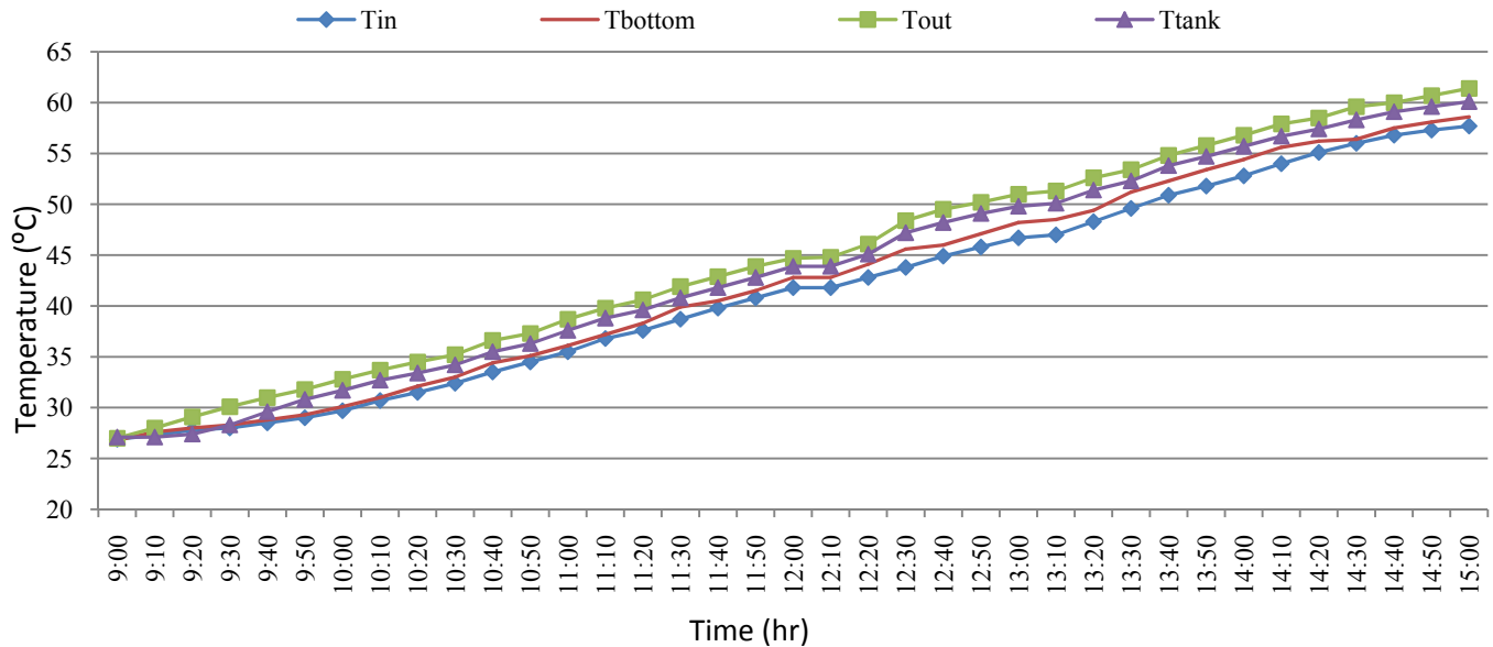
Fig. 12: Temperature of system 3 at 22° on November 22, 2014
