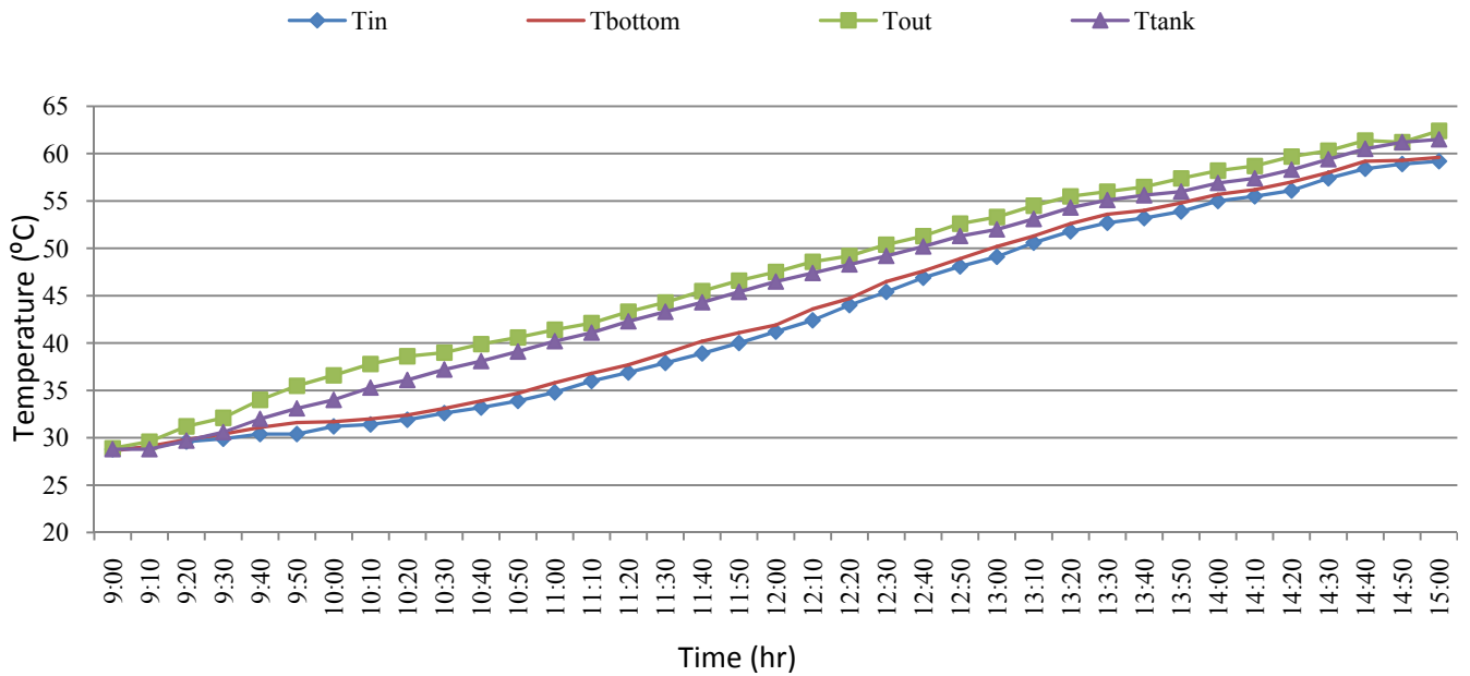
Fig. 15: Temperature of SWH3 at 45° on November 24, 2014
