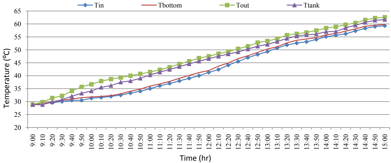
Fig. 14: Temperature of SWH2 at 45° on November 24, 2014
