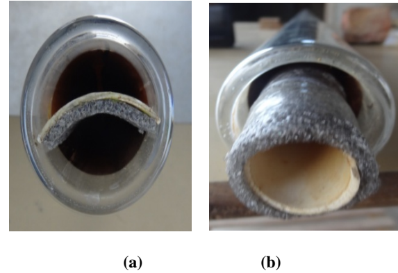
Fig. 5: (a) Curved insulated surface (b) concentric circular insulated surface
