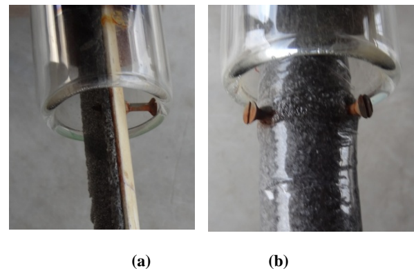
Fig. 6: (a) Position of support on curved insulated surface (b) Position of supports on concentric circular insulated surface
