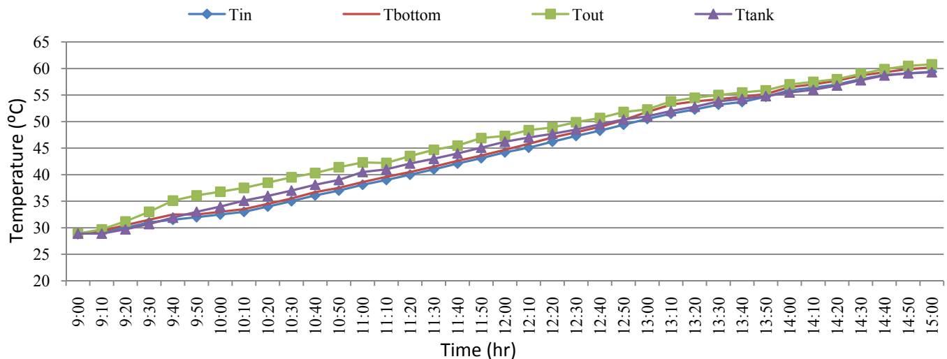
Fig. 13: Temperature of SWH1 at 45° on November 24, 2014
