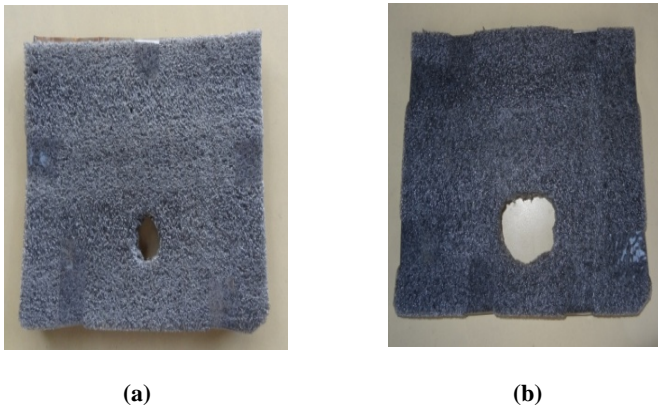
Fig. 4: (a) photograph of parting wall of SWH2 (b) photograph of parting wall of SWH3
